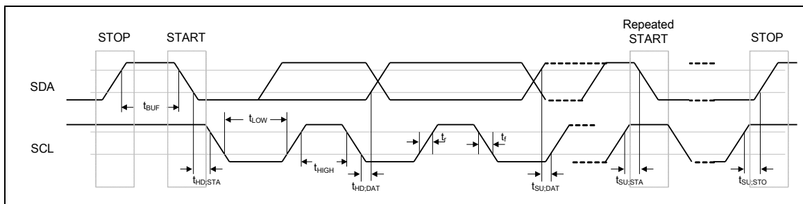
Figure 5.9-1 Bus Timing
